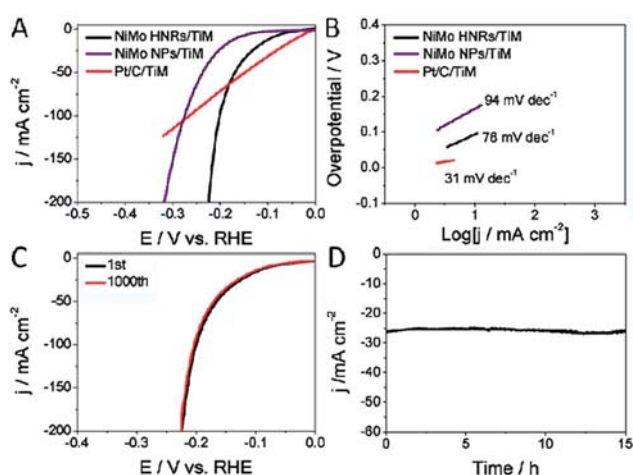
Fig. 3 (A) Polarization curves of NiMo HNRs/TiM, NiMo NPs/TiM, and Pt/C/TiM with a scan rate of 2 \text{ mV s}^{-1} in 1.0 M KOH. (B) The corresponding Tafel plots. (C) Polarization curves of NiMo HNRs/TiM initially and after 1000 CV scanning between +0.1 and -0.2 \text{ V} vs. RHE. (D) Time-dependent current density curve of NiMo HNRs/TiM under a static overpotential of 140 mV for 15 h.
