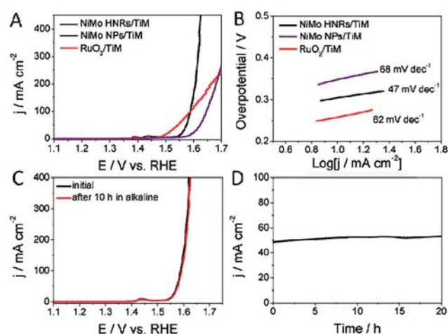
Fig. 2 (A) Polarization curves of NiMo HNRs/TiM, NiMo NPs/TiM and RuO 2 /TiM with a scan rate of 2 mV s -1 in 1.0 M KOH. (B) The corresponding Tafel plots. (C) Polarization curves of NiMo HNRs/TiM initially and after chronopotentiometric electrolysis of 10 h. (D) Time-dependent current density curve of NiMo HNRs/TiM under a static overpotential of 350 mV for 20 h.
