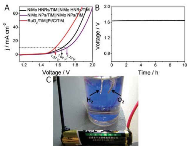
Fig. 4 (A) Polarization curves of water electrolysis for NiMo HNRs/TiM||NiMo HNRs/TiM, NiMo NPs/TiM||NiMo NPs/TiM, and \text{RuO}_2/\text{TiM} ||Pt/C/TiM with a scan rate of 2 \text{ mV s}^{-1} in 1.0 M KOH. (B) Chronopotentiometric curve of water electrolysis for NiMo HNRs/TiM||NiMo HNRs/TiM with a constant current density of 10 \text{ mA cm}^{-2} . (C) The NiMo HNRs/TiM||NiMo HNRs/TiM water splitting system driven by an \sim 1.5 \text{ V} AAA battery.
